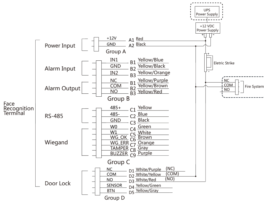
Figure 4-8 Device Wiring
