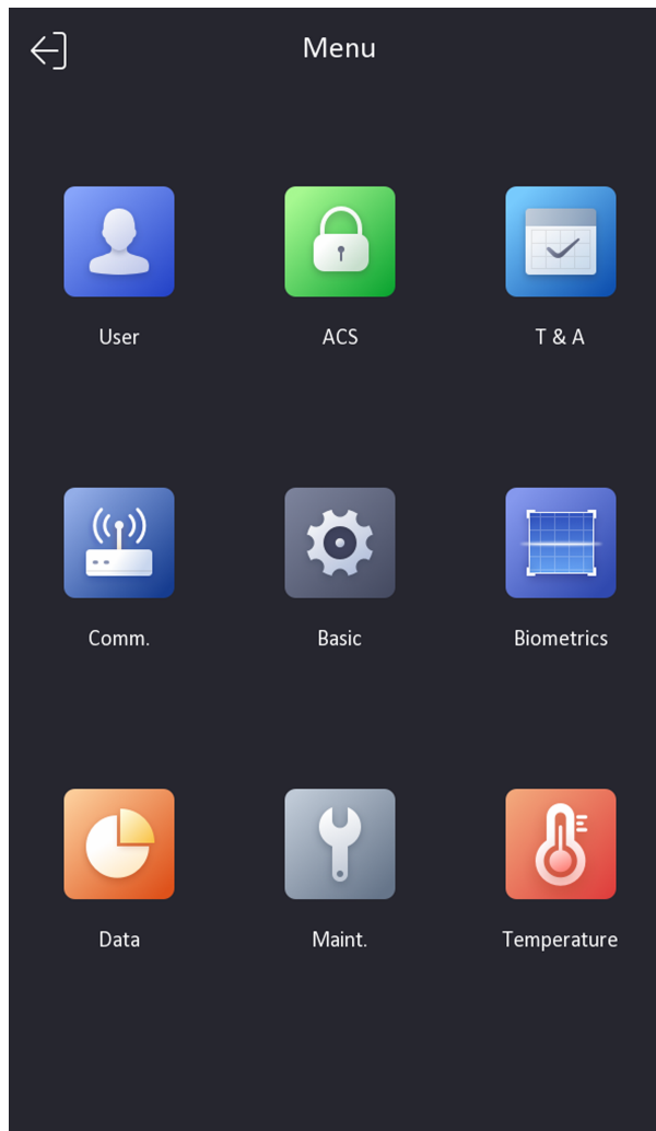
Figure 7-3 Home Page
