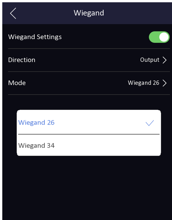
Figure 7-6 Wiegand Settings
