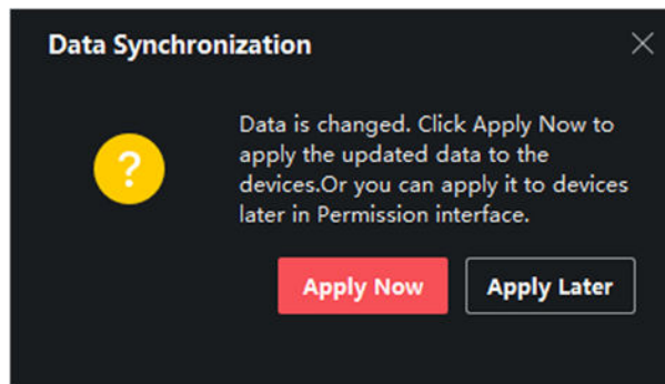
Figure 9-10 Data Synchronization
