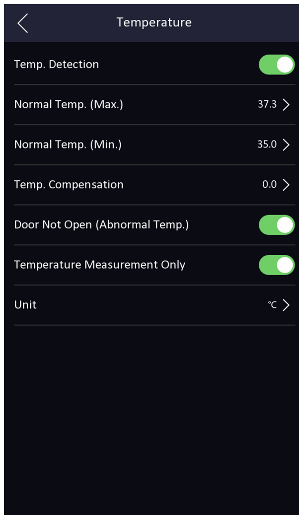
Figure 7-16 Temperature Measurement Parameters
