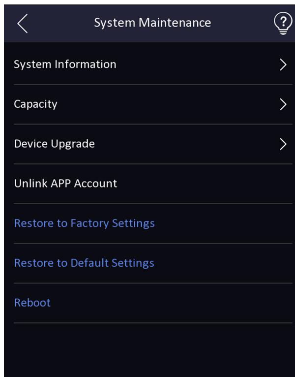
Figure 7-15 Maintenance Page
