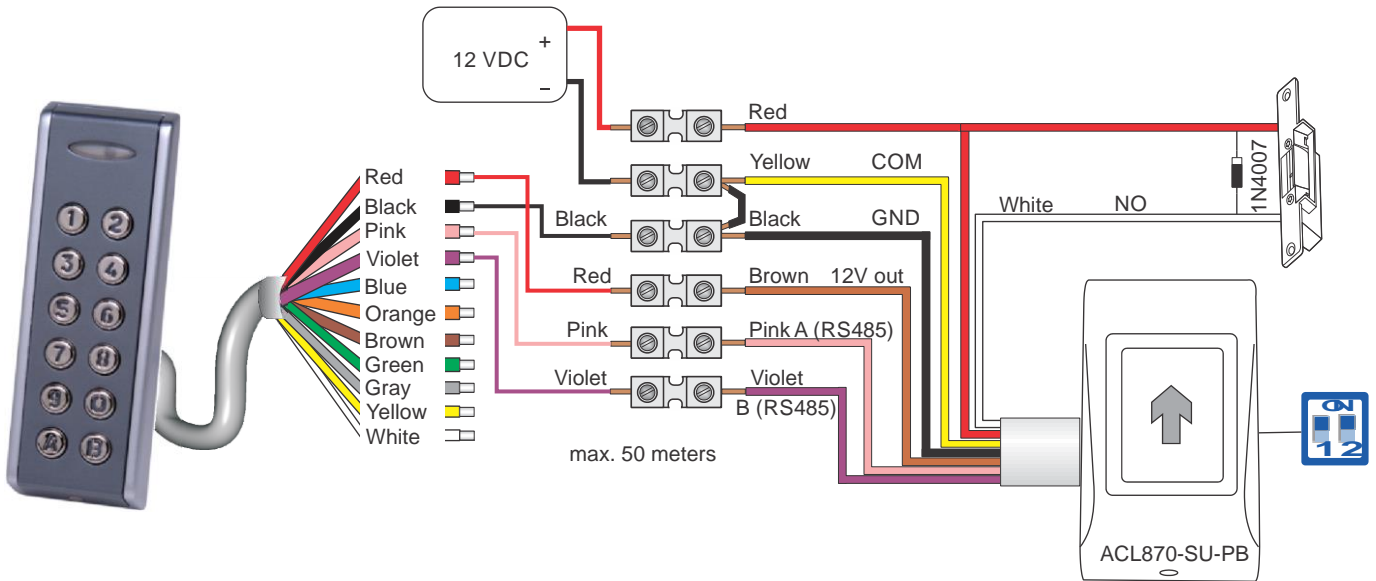
Figure 4: Keypad wiring
